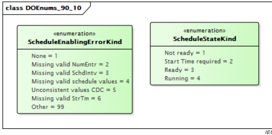
Figure 9 – Class diagram DOEnums_90_10::DOEnums_90_10
