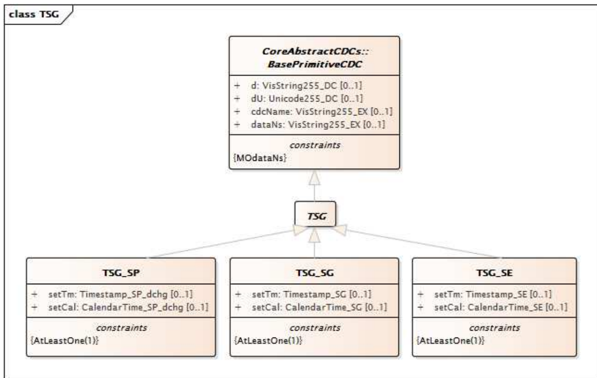
Figure D.2 – Class diagram TSG::TSG
